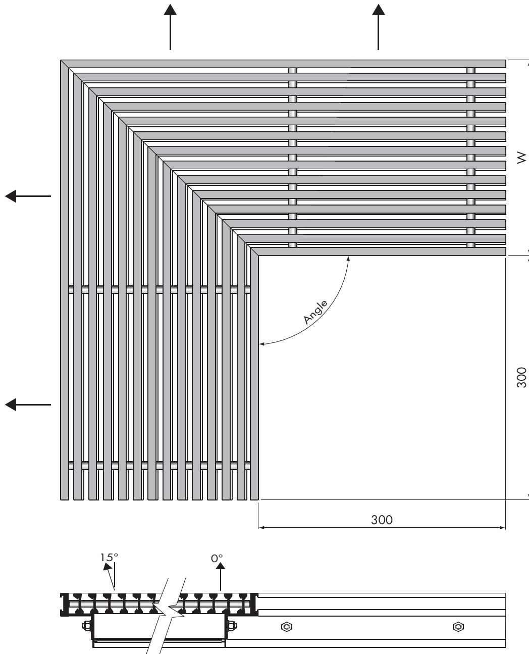
HDFG-L - Linear Corner Sections
