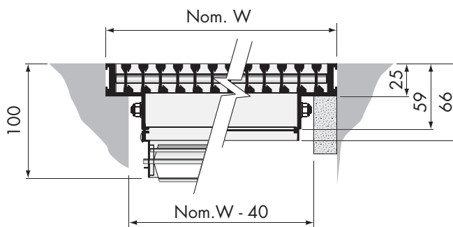
Intermediate section
